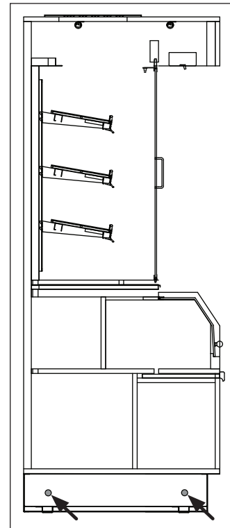
Fig. 5 Bolt locations (BWU-RB-D)
